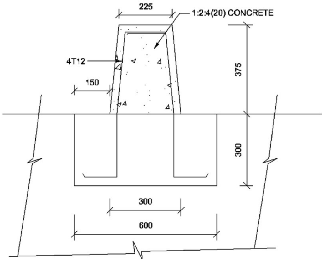
SECTION B-B
